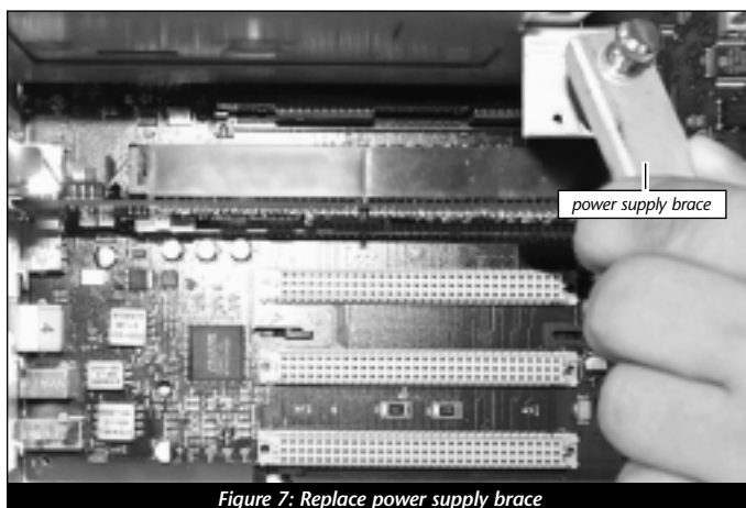
Figure 7: Replace power supply brace
