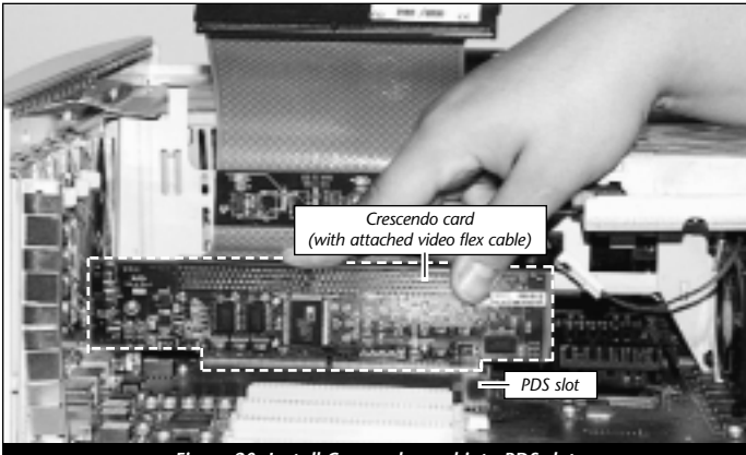
Figure 20: Install Crescendo card into PDS slot
