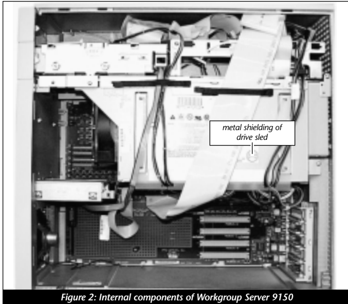
Figure 2: Internal components of Workgroup Server 9150
