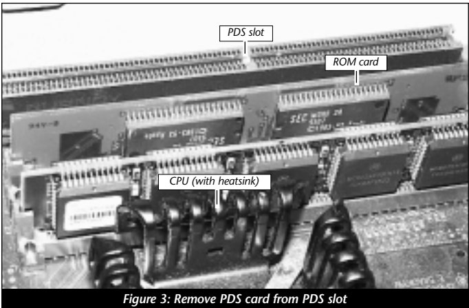
Figure 3: Remove PDS card from PDS slot
