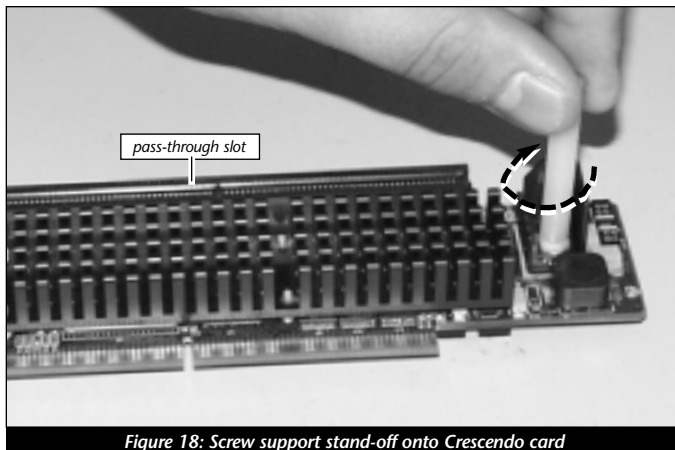
Figure 18: Screw support stand-off onto Crescendo card
